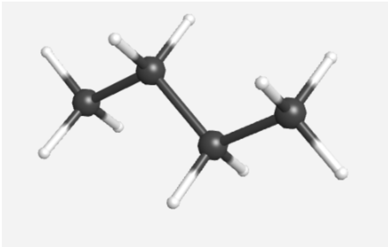
Butane (student model)
