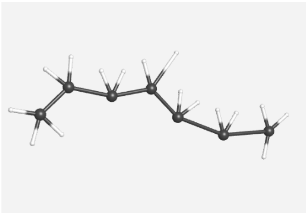
Heptane (student model)
