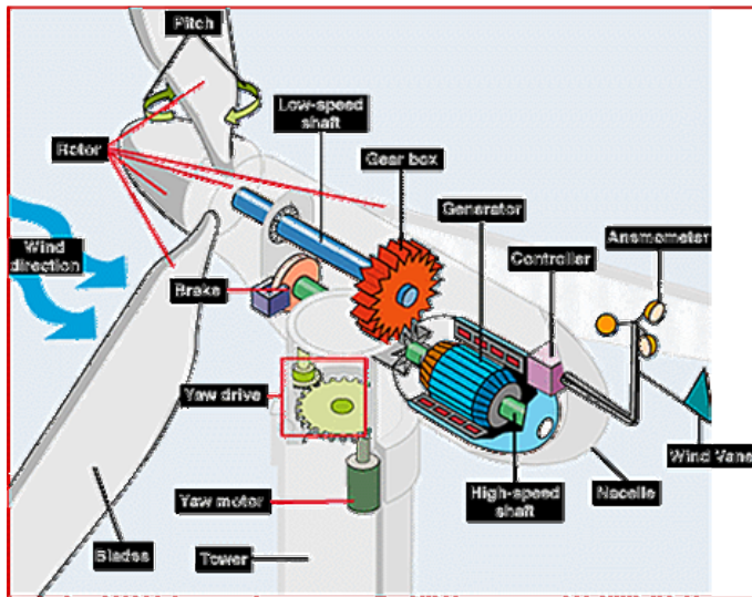
Fig. 1 The components of a common horizontal-axis turbine
