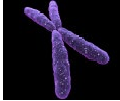
X chromosome
