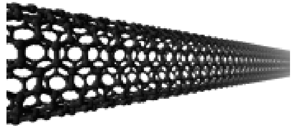
carbon nanotube
