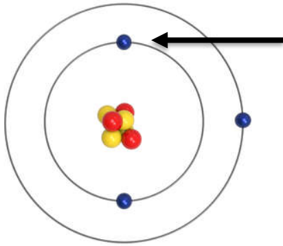
single electron
