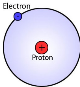
hydrogen atom
